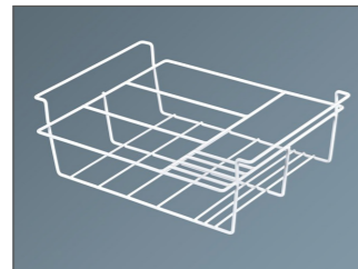
SCOOP BASKET: ONLY FOR MOBILUX 11 KURVSCOOPF3+1 W X H: 442 X 123 MM
